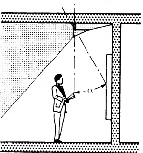
⑨ Wall illumination, floodlight
